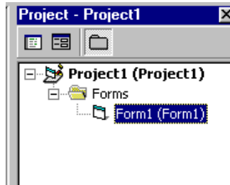
Gambar 1.8 Project Explorer
