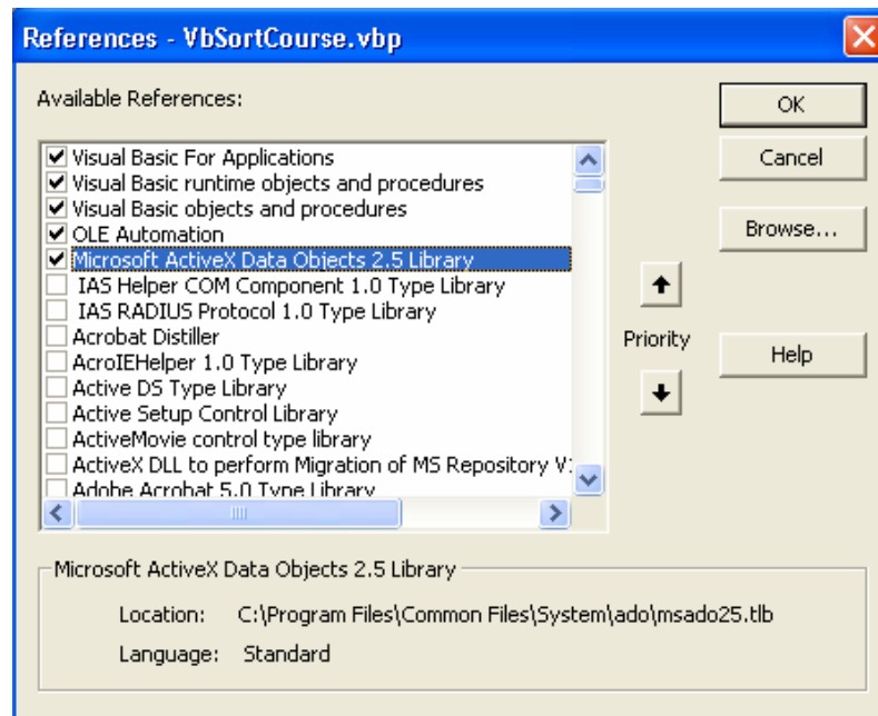
Gambar 4.10 Window References
