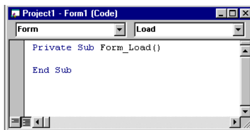
Gambar 1.7 Code Window
