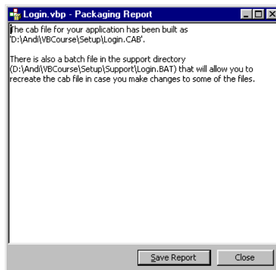
Gambar 1.27 Tampilan Report
