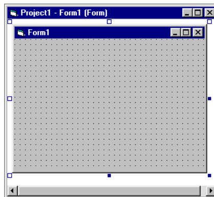
Gambar 1.6 Form
