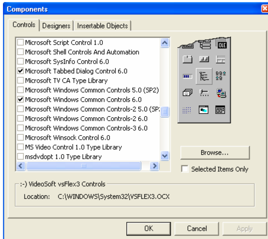
Gambar 4.9 Window Components
